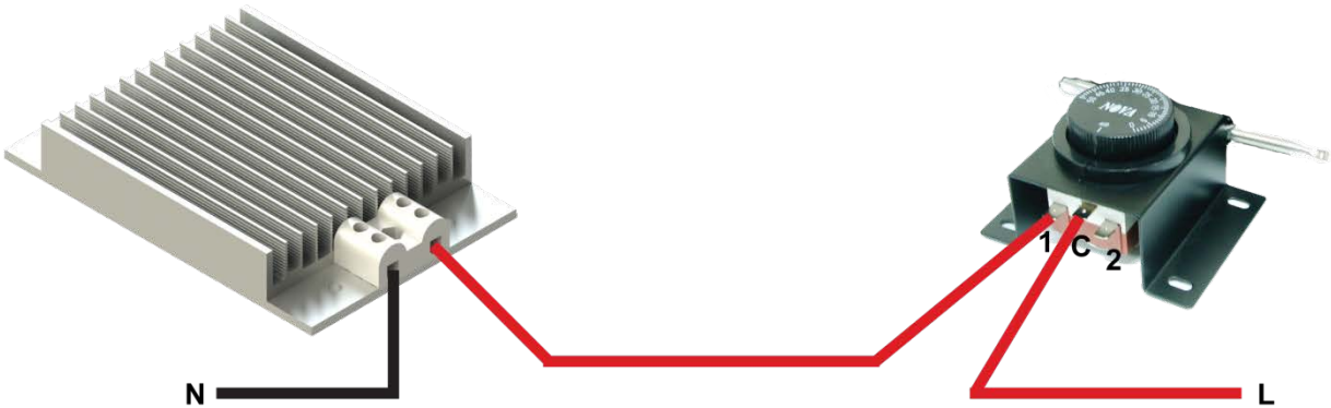
Wiring sample
