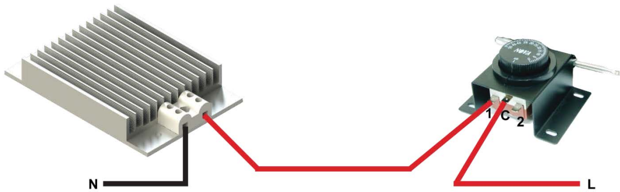
Wiring sample
